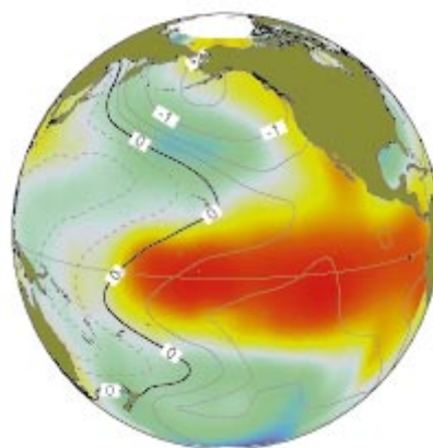
FIG. 2. COADS SST (color shaded) and SLP (contoured) regressed upon (a) the PDO index and (b) the CTI for the period of record 1900–92. Contour interval is 1 mb, with additional contours drawn for \pm 0.25 and 0.50 mb. Positive (negative) contours are dashed (solid).
