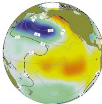
(a) SST and SLP regressed on the PDO index
